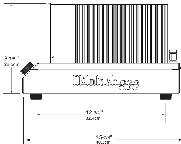
Figure 01– MC830 Dimensions
