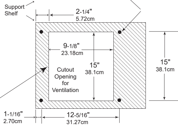
Figure 02– Custom cutout dimensions
