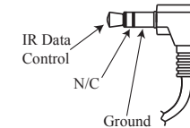
Figure 06– IR 3.5mm connector
