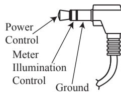
Figure 08– Power control (trigger) mini plug
