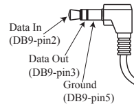
Figure 04– Mini plug for RS232 connection
