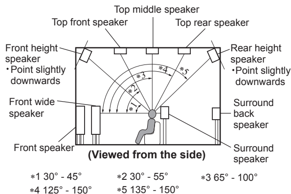
Figure 18– Speaker angles
