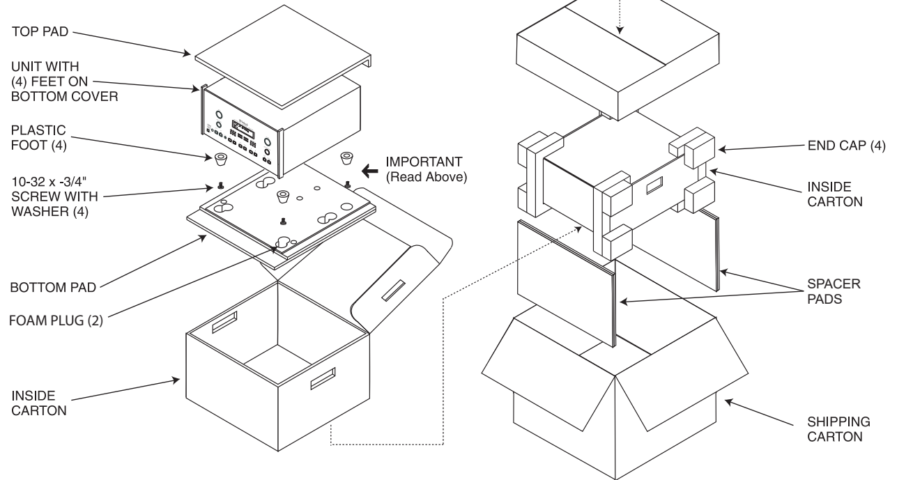
Figure 28– Re-packing diagram
