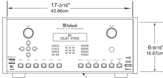
MX123 Front Panel Custom Cabinet Cutout
