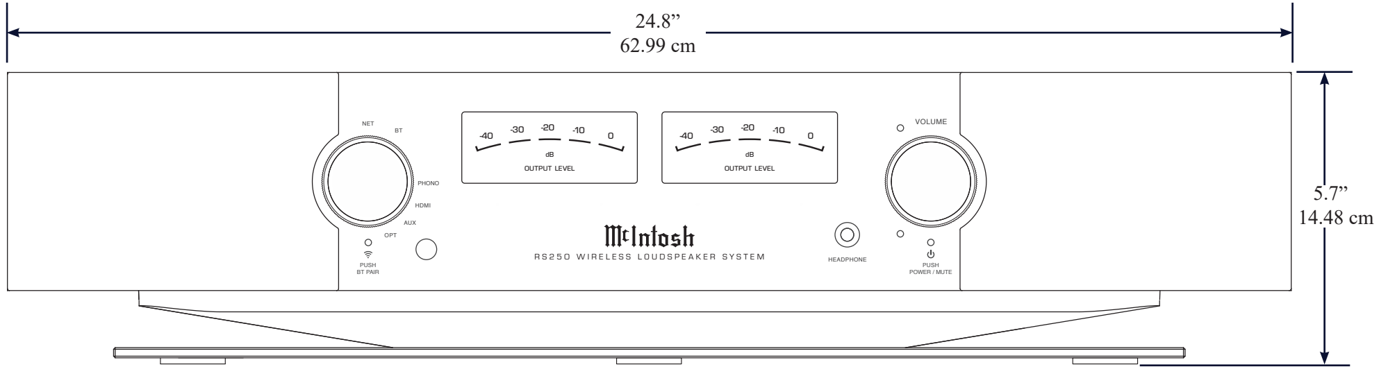
Figure 6– Front View
